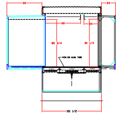
FRONT VIEW ILLUSTRATING CHASSIS STRUCTURE AS IT RELATES TO CABLE PATH.
