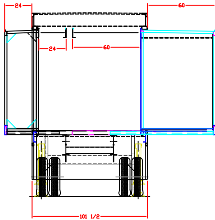
REAR VIEW ILLUSTRATING CHASSIS STRUCTURE AS IT RELATES TO CABLE PATH.
